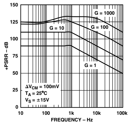
TPC 10. Positive PSRR vs. Frequency
