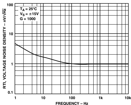
TPC 2. Voltage Noise Density vs. Frequency
