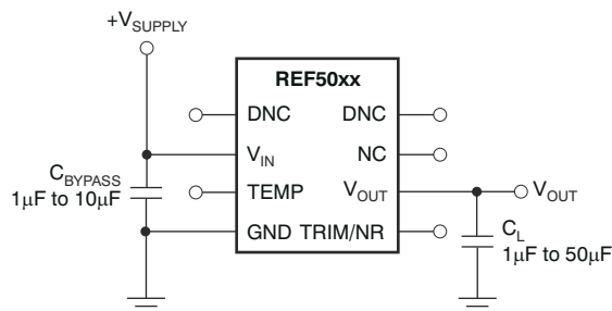
Figure 9-4. Basic Connections
