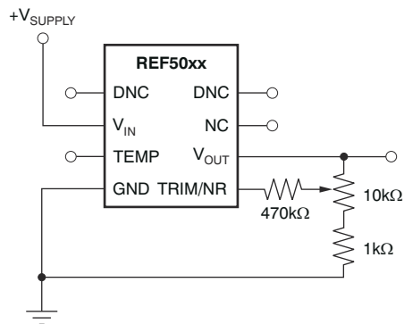
Figure 9-3. V OUT Adjustment Using the TRIM/NR Pin
