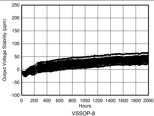
Figure 7-24. REF50xx Long-Term Stability (First 2000 Hours)
