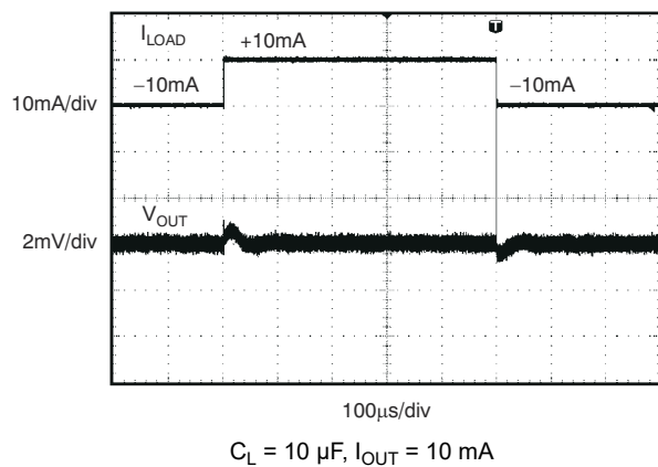
Figure 7-19. Load Transient
