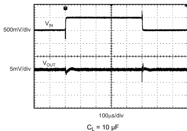
Figure 7-21. Line Transient
