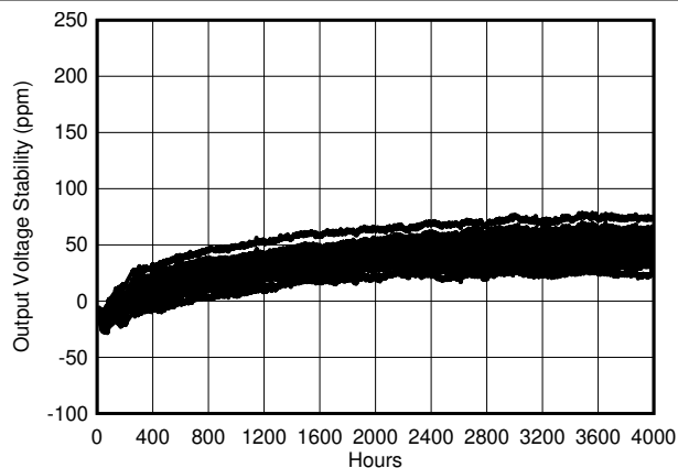
Figure 7-26. REF50xx Long-Term Stability (4000 Hours)
