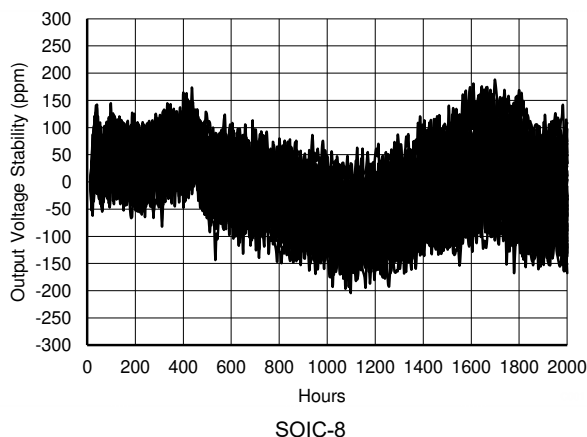
Figure 7-29. REF50xx Long-Term Stability (2000 Hours)
