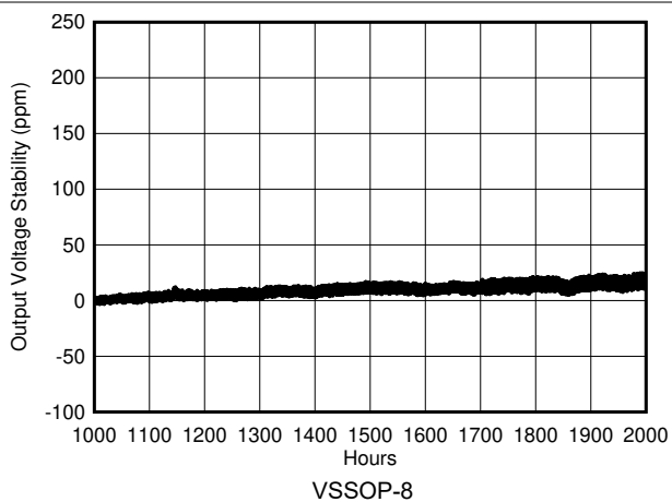
Figure 7-23. REF50xx Long-Term Stability (Second 1000 Hours)
