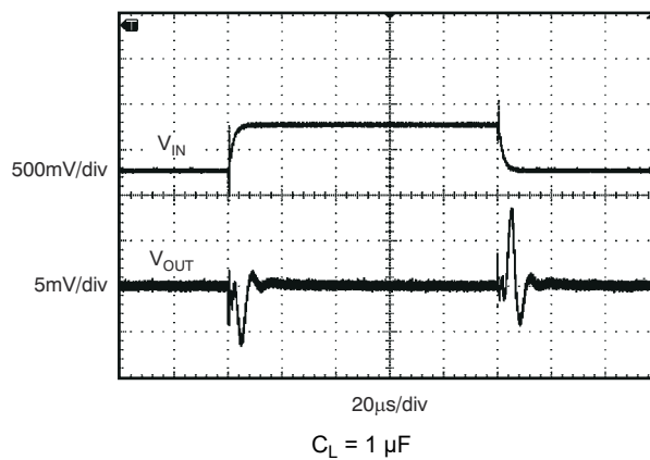
Figure 7-20. Line Transient
