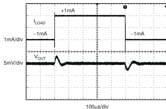
Figure 7-16. Load Transient
