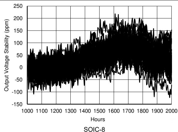
Figure 7-28. REF50xx Long-Term Stability (Second 1000 Hours)
