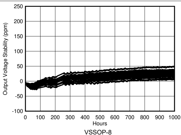
Figure 7-22. REF50xx Long-Term Stability (First 1000 Hours)
