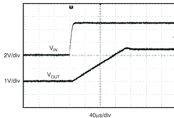
Figure 7-14. Start-Up
