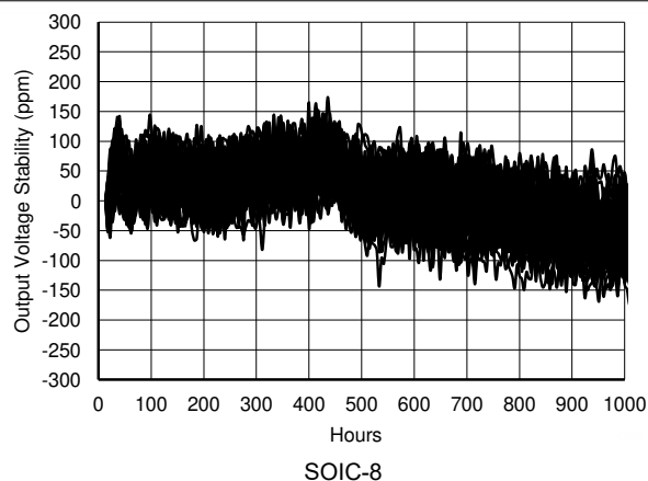
Figure 7-27. REF50xx Long-Term Stability (First 1000 Hours)
