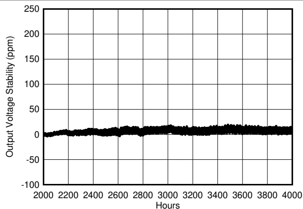
Figure 7-25. REF50xx Long-Term Stability (Second 2000 Hours)
