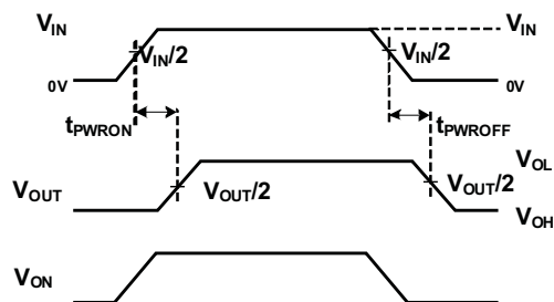
Figure 21. t_{PWON}/t_{PWROFF} Waveforms
