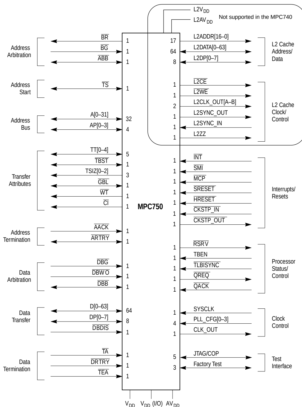
Figure 4. MPC750 Microprocessor Signal Groups
