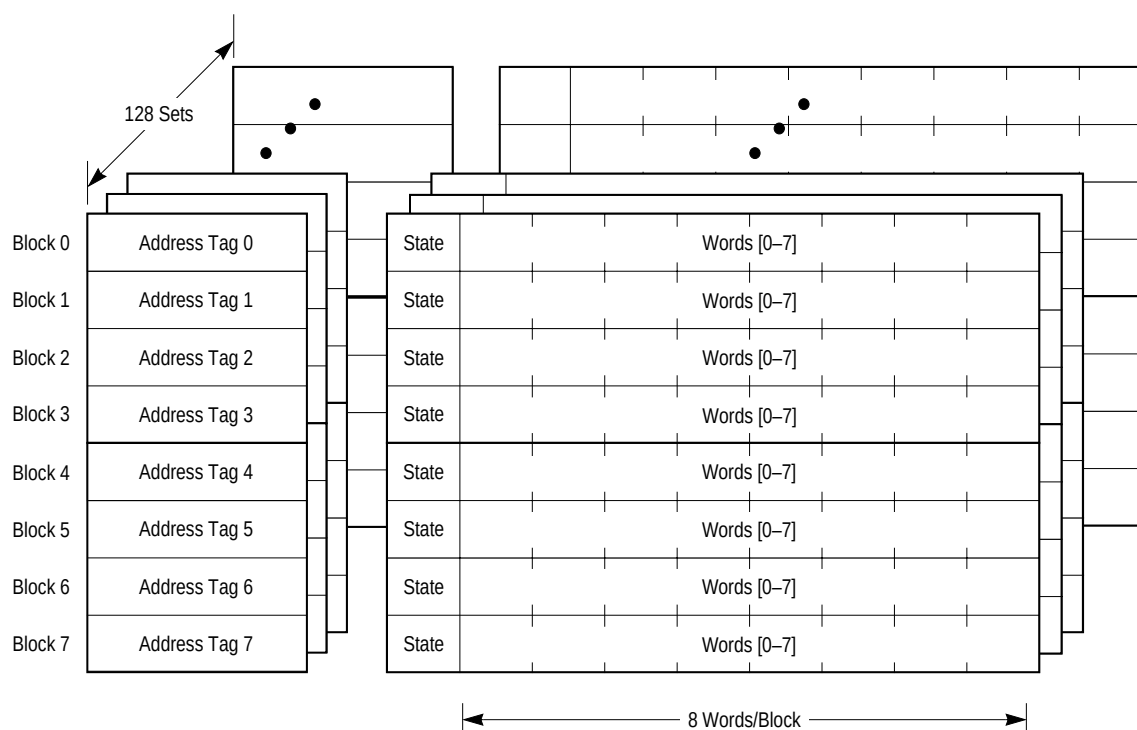
Figure 2. Cache Organization
