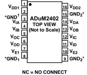
Figure 7. ADuM2402 Pin Configuration
