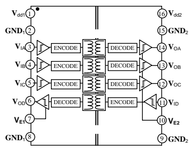
Figure 2. ADuM2401 Functional Block Diagram
