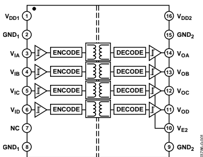
Figure 1. ADuM2400 Functional Block Diagram
