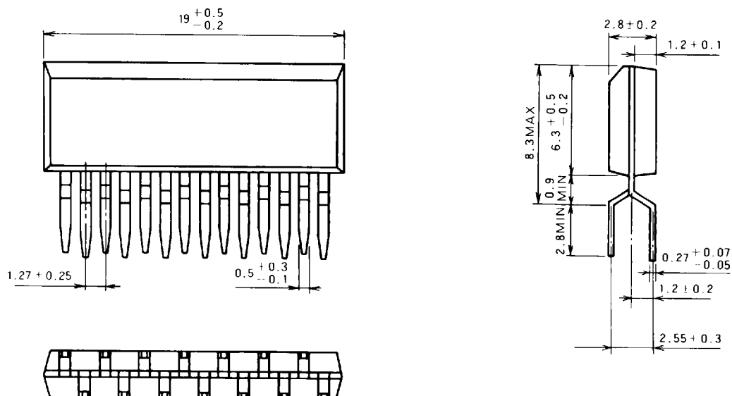
TYPE 14P5A 14-PIN MOLDED PLASTIC ZIP
