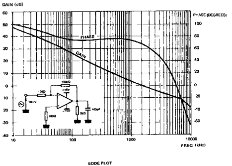
BODE PLOT
