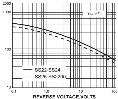
FIG. 5-TYPICAL JUNCTION CAPACITANCE
