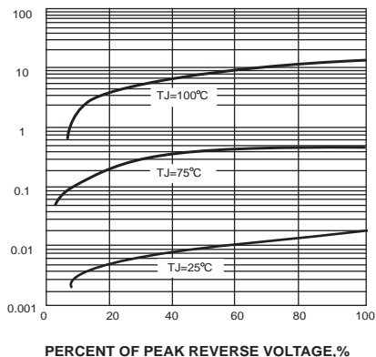
FIG. 4-TYPICAL REVERSE CHARACTERISTICS
