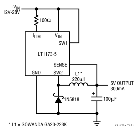
+20V to 5V Step-Down Converter
