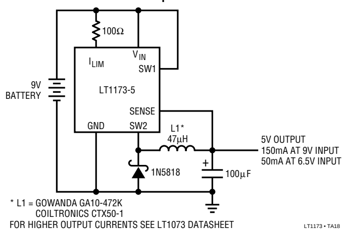
9V to 5V Step-Down Converter
