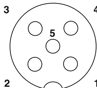
Pin assignment of M12 socket, 5-pos.
