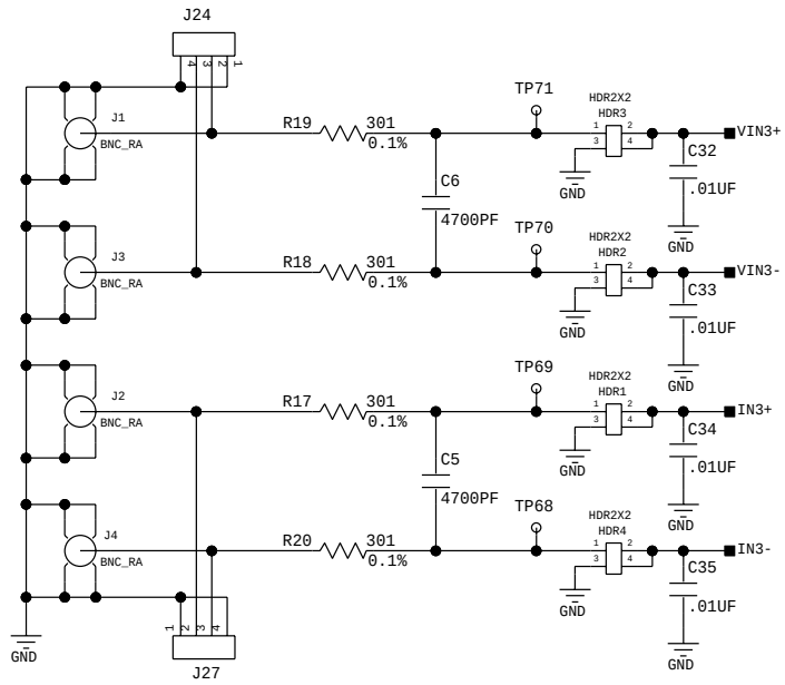
Figure 2. Analog Inputs
