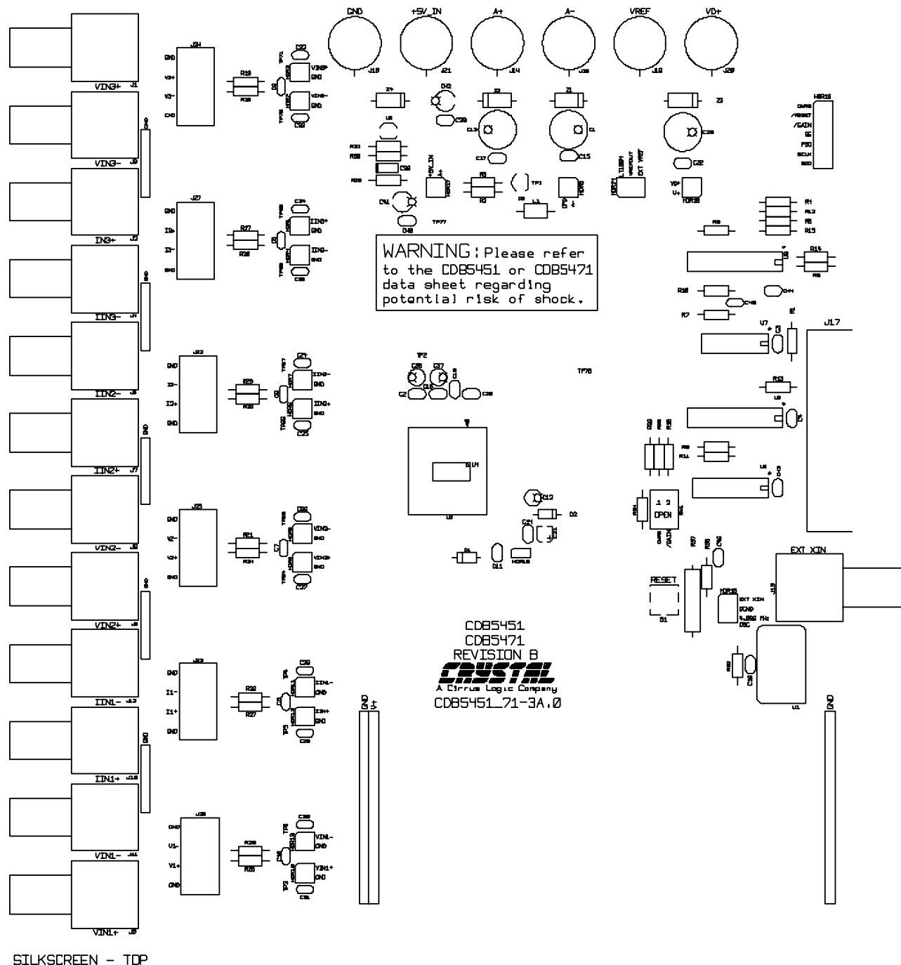
Figure 10. Silkscreen
