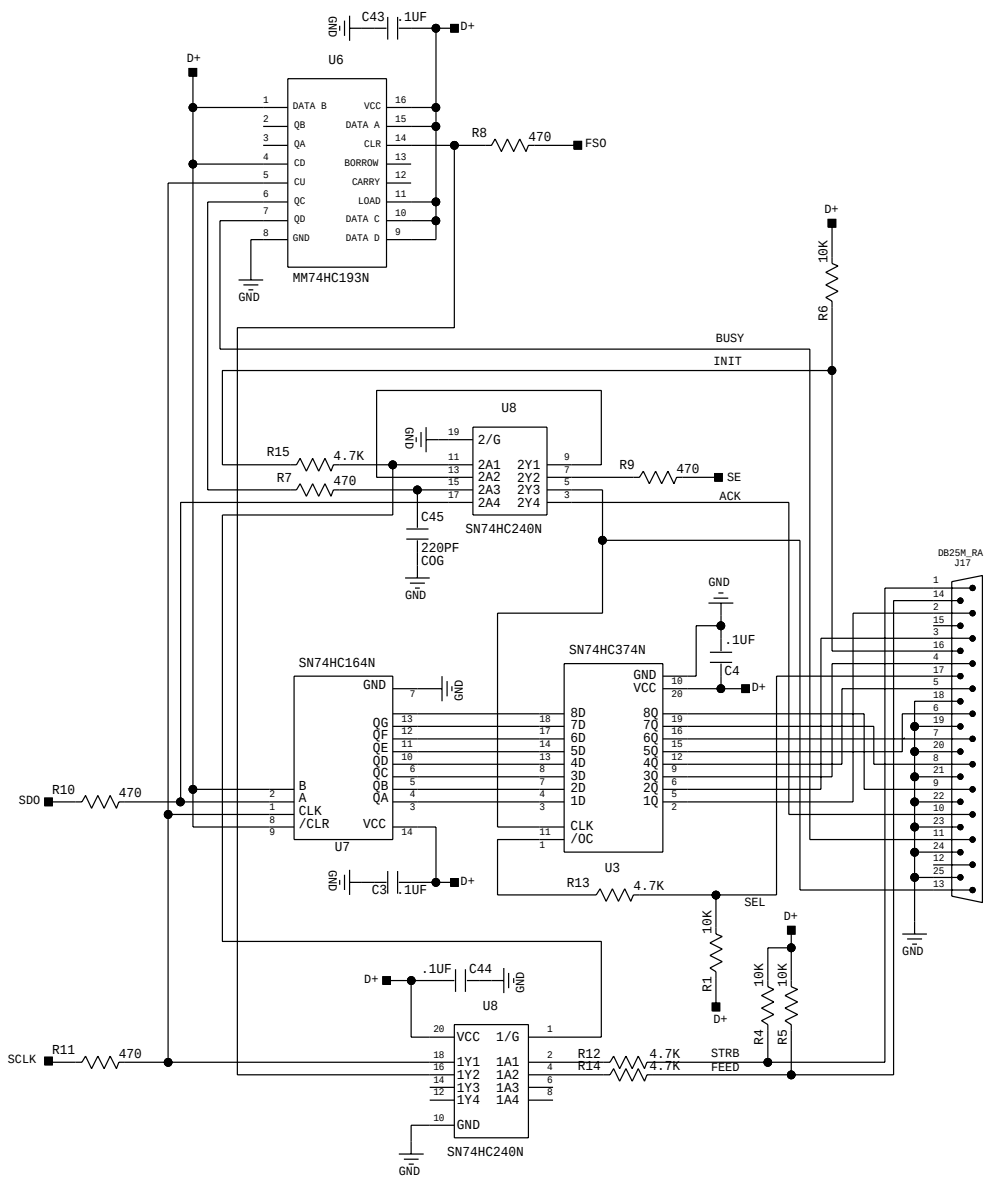
Figure 3. Digital Circuitry
