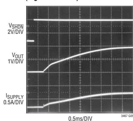
Start-Up Waveform (Figure 2 Circuit)
