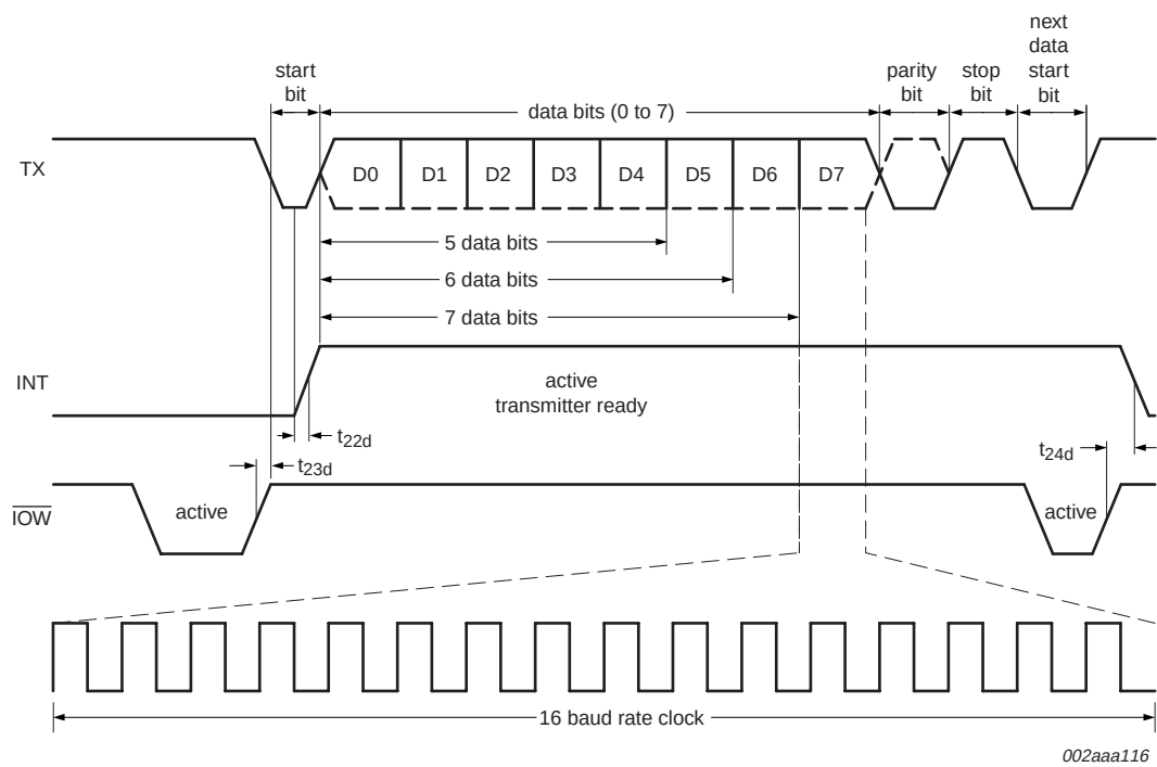
Fig 17. Transmit timing
