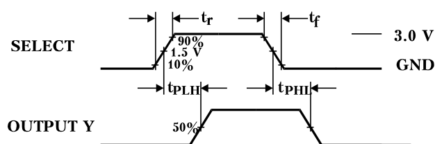
Figure 2. Switching Waveforms
