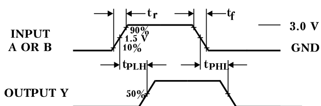
Figure 1. Switching Waveforms
