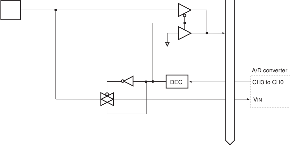
Figure B.27 Port B Block Diagram (PB7 to PB0)
