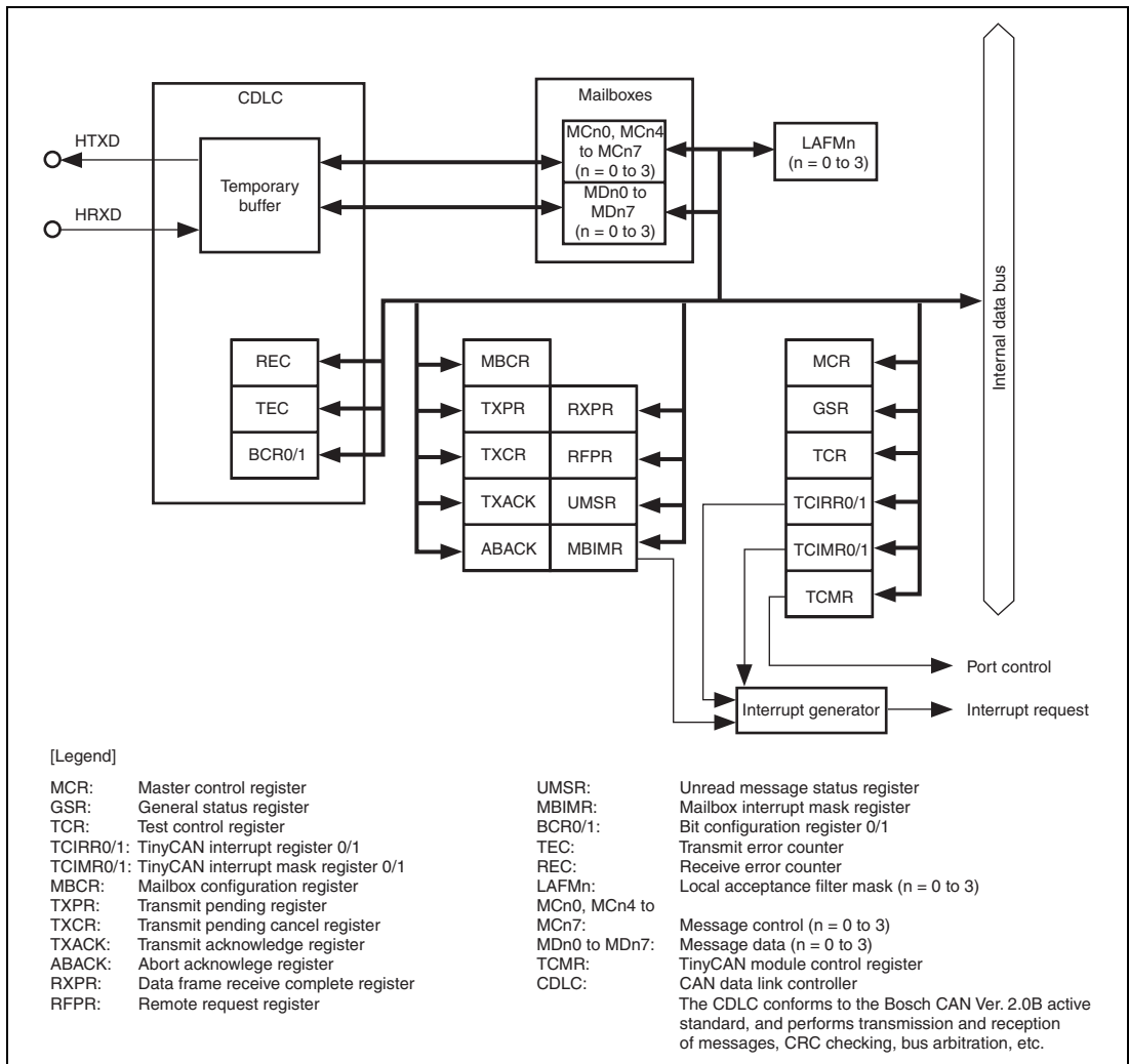
Figure 15.1 TinyCAN Block Diagram
