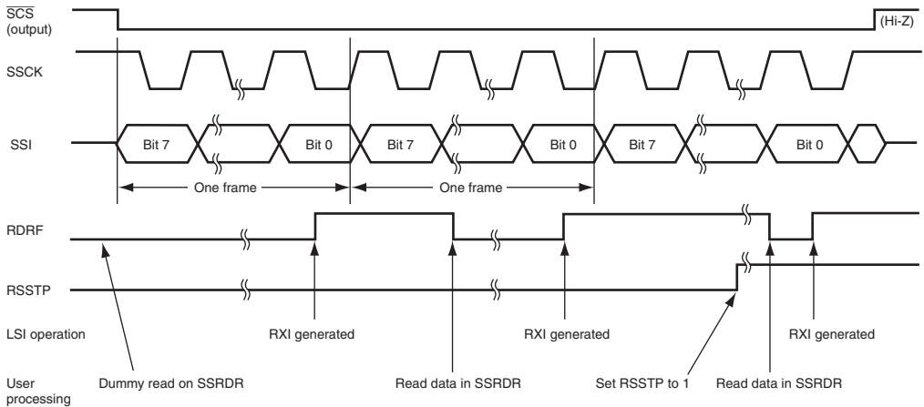
Figure 16.12 Example of Operation in Data Reception (MSS = 1)
