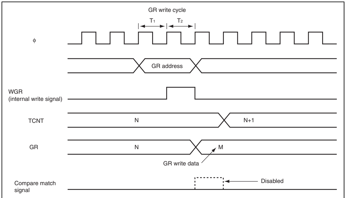
Figure 12.54 Contention between GR Write and Compare Match
