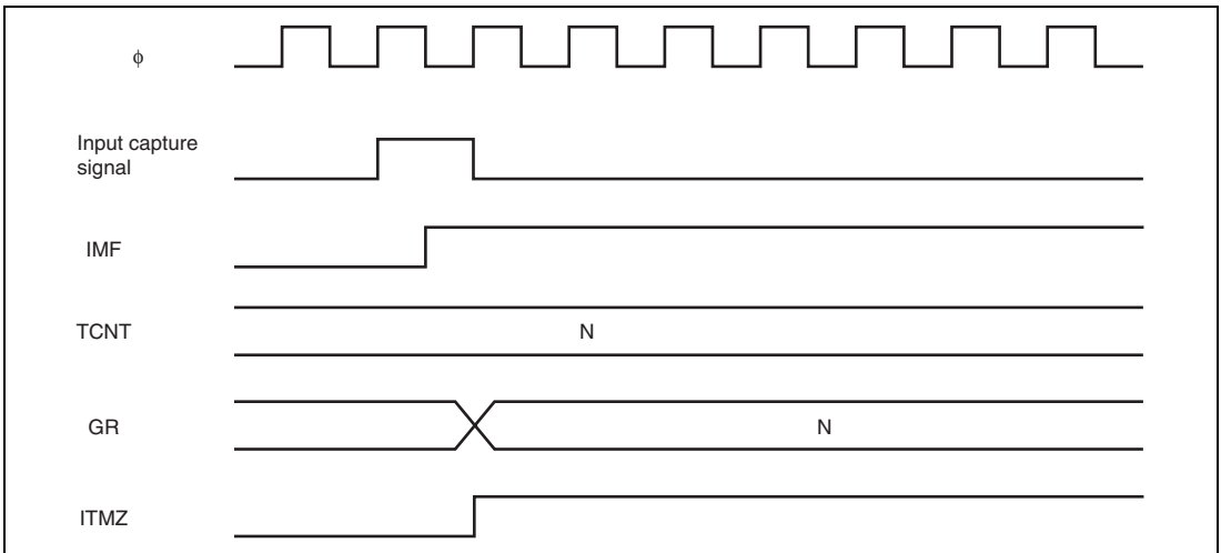
Figure 12.49 IMF Flag Set Timing at Input Capture
