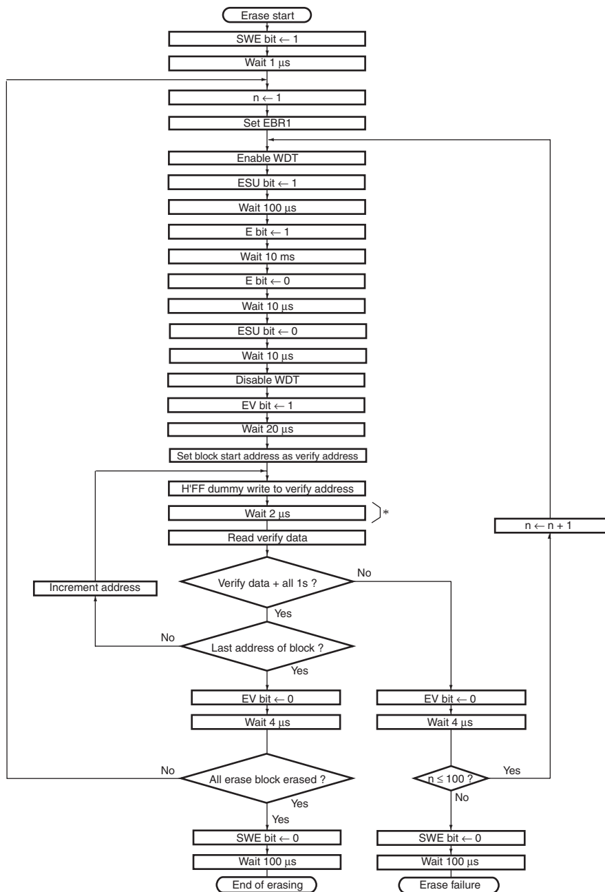
Figure 7.4 Erase/Erase-Verify Flowchart
