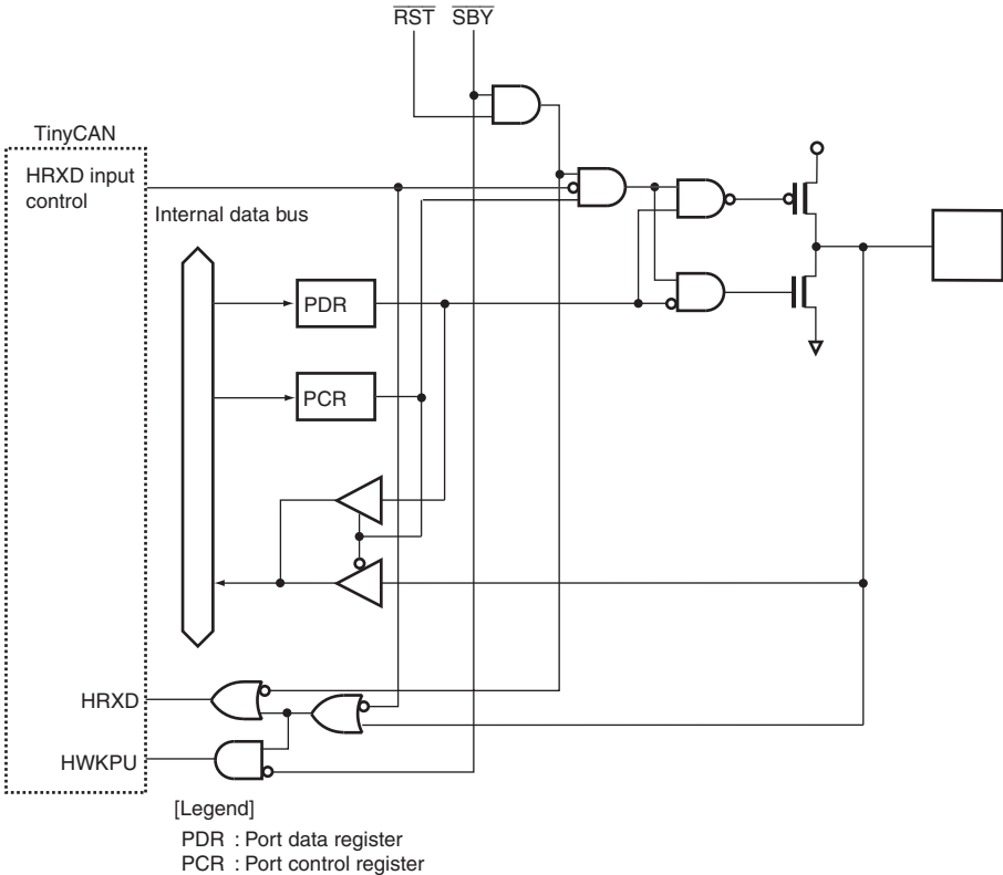
Figure B.21 Port 9 Block Diagram (P96)
