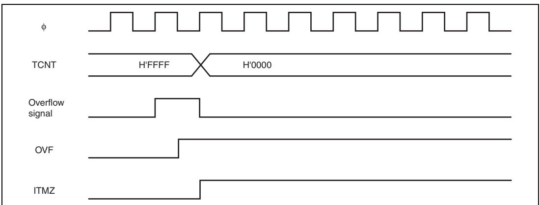
Figure 12.50 OVF Flag Set Timing
