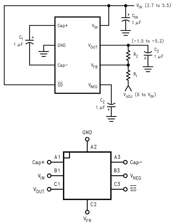
8-Bump DSBGA (Top View)
