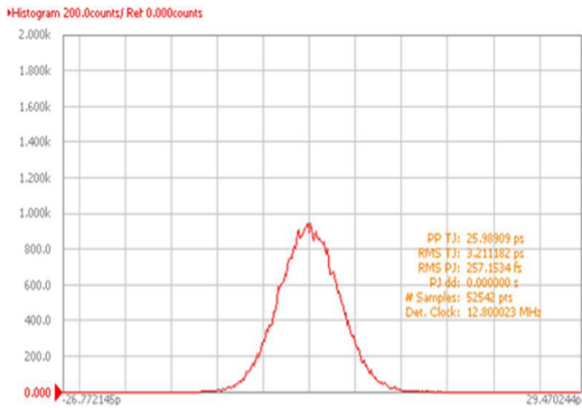
Frequency - 12.288MHz
