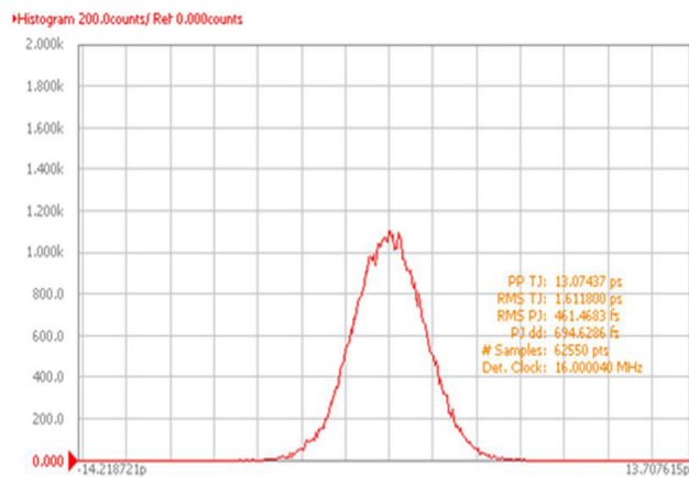
Frequency - 16.000MHz
