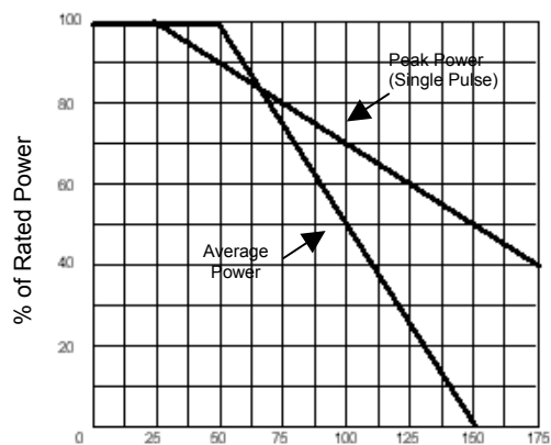
FIGURE 2 Lead Length = 3/8"
