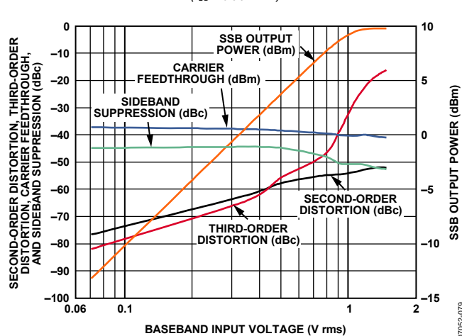
Figure 39. Second- and Third-Order Distortion, Carrier Feedthrough, Sideband Suppression, and SSB P_{OUT} vs. Baseband Differential Input Level ( f_{LO} = 2150 MHz)
