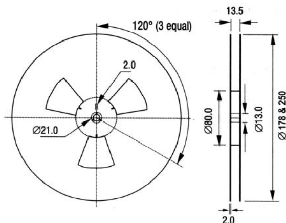
Outline in mm - Reel
