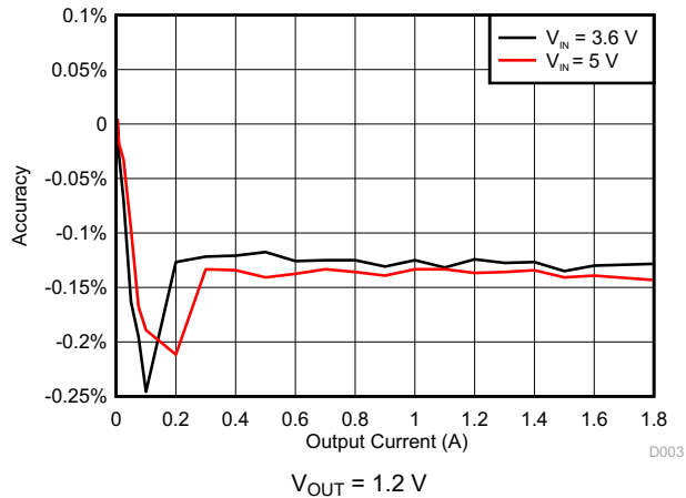
图 7-3. DCDC3 Accuracy
