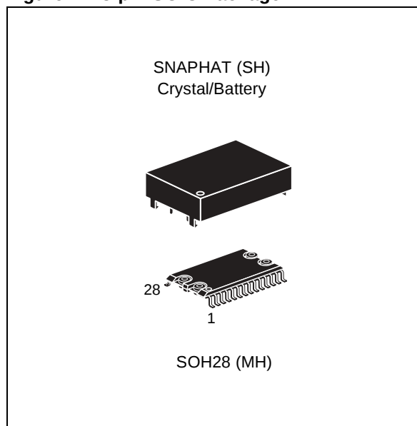
Figure 2. 28-pin SOIC Package
