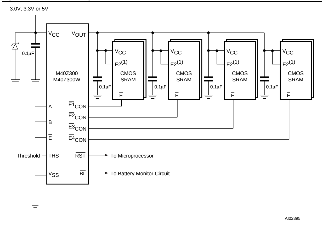
Figure 7. Hardware Hookup
