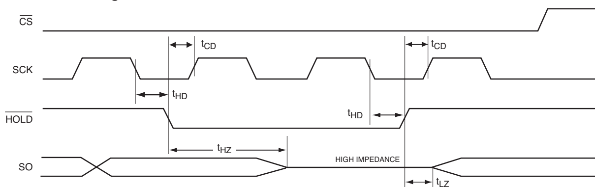
Figure 2. HOLD Timing
