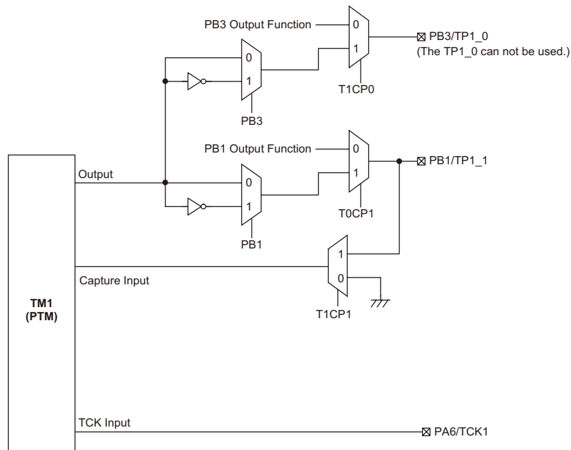
TM1 Function Pin Control Block Diagram
