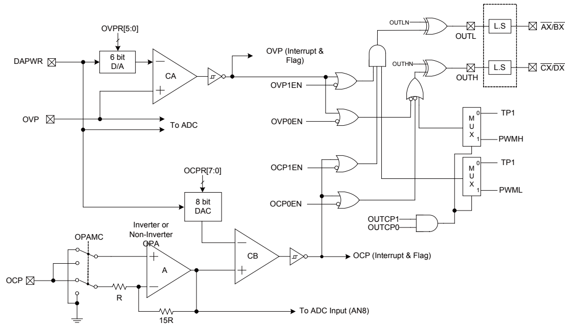
Over Voltage and Over Current Protection Block Diagram
