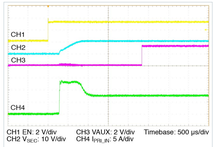
Figure 15 — Start up from application of EN with pre-applied V_{PRI\_DC} = 54 V, 20% I_{SEC\_DC} , 100% C_{SEC\_OUT\_EXT}
