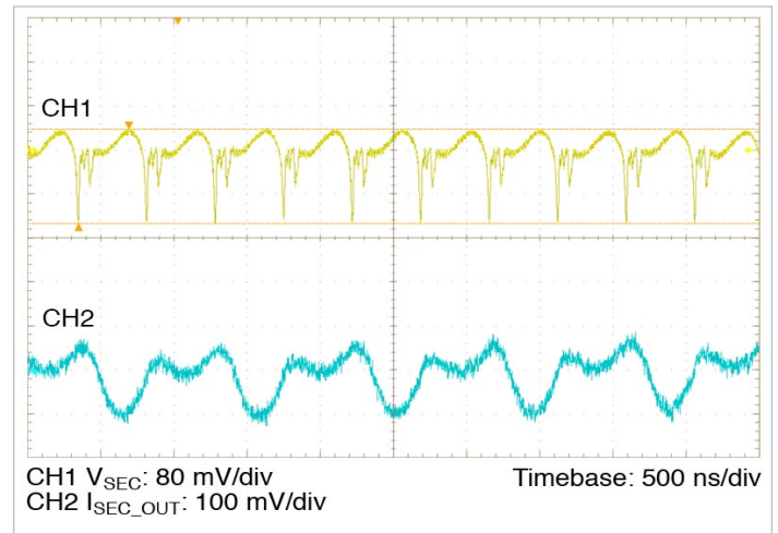
Figure 11 — Full load ripple, 270 \mu F C_{PRI\_OUT\_EXT} ; No external C_{SEC\_OUT\_EXT} . Board mounted module, scope setting : 20 MHz analog BW
