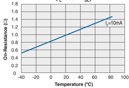
CPC1788 Typical On-Resistance vs. Temperature ( I_L=250\text{mA}_{\text{DC}} )
