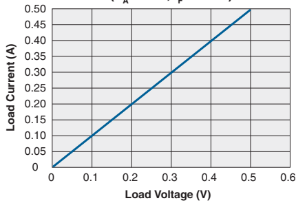
CPC1788 Typical Load Current vs. Load Voltage ( T_A=25^\circ\text{C} , I_F=10\text{mA} )
