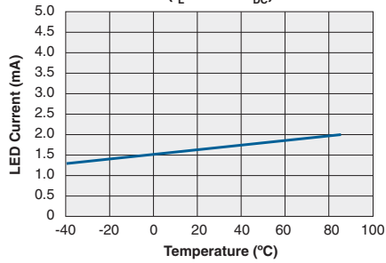
CPC1788 Typical I_F for Switch Operation vs. Temperature ( I_L=250\text{mA}_{\text{DC}} )
