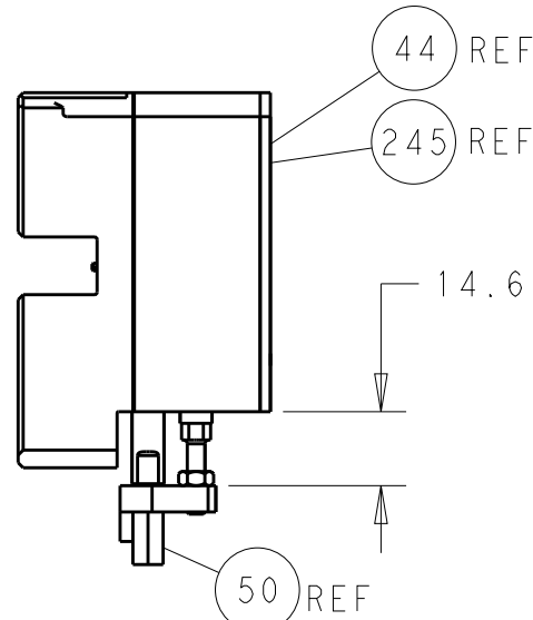
HOLDDOWN SET-UP
