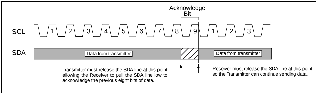
FIGURE 6-2: ACKNOWLEDGE TIMING
