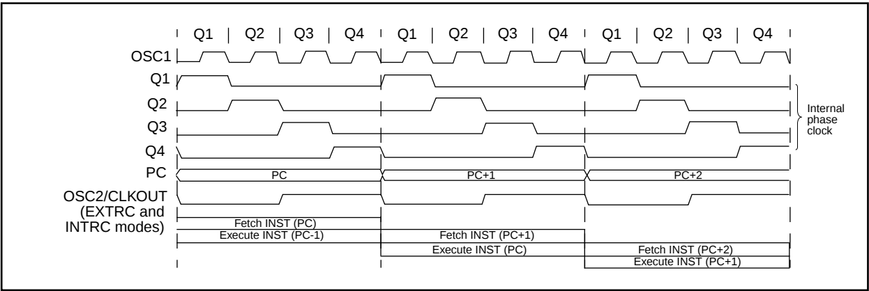
FIGURE 3-2: CLOCK/INSTRUCTION CYCLE
