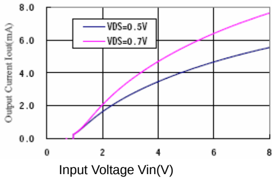
(6) PCH Driver Output Current VS. Input Current Detector threshold=0.9V
