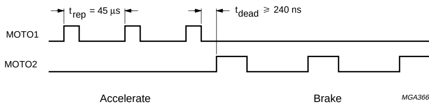
Fig.17 Motor 2-line PWM mode timing.
