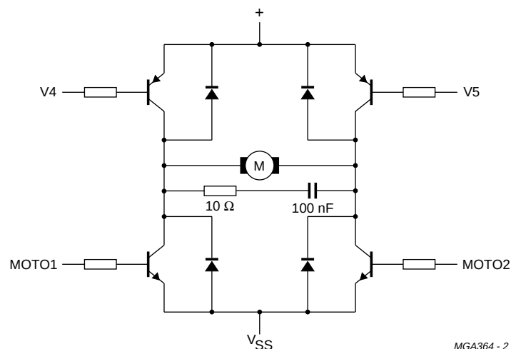
Fig.20 Motor 4-line PWM mode application diagram.
