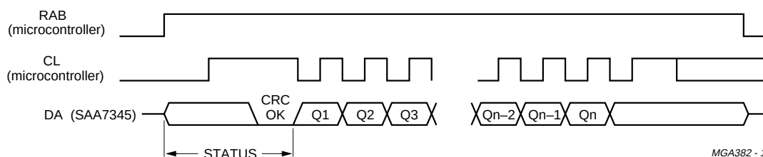
Fig.8 SAA7345 Q-channel subcode READ timing.
