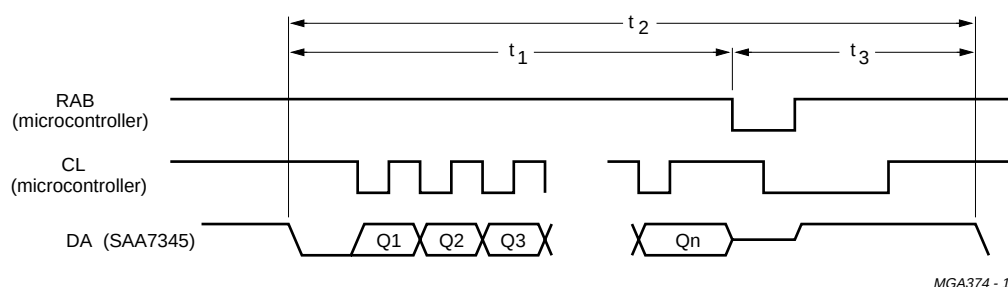
Fig.10 SUBQREADY-I timing when subcode is being read.
