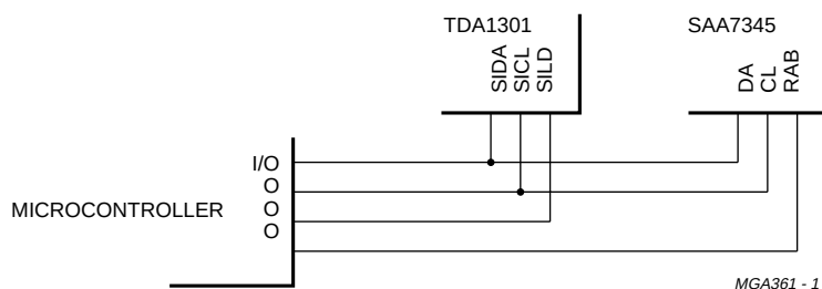
Fig.11 SAA7345 microcontroller interface application diagram.
