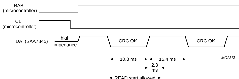
Fig.9 SUBQREADY-I timing when no subcode is read.
