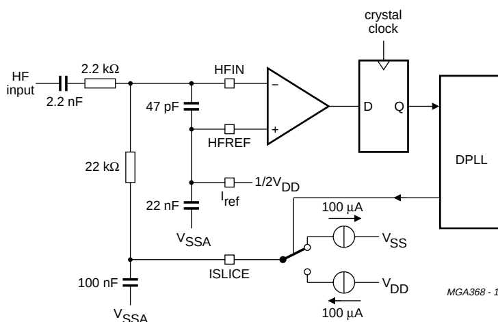
Fig.3 Data slicer showing typical application components.
