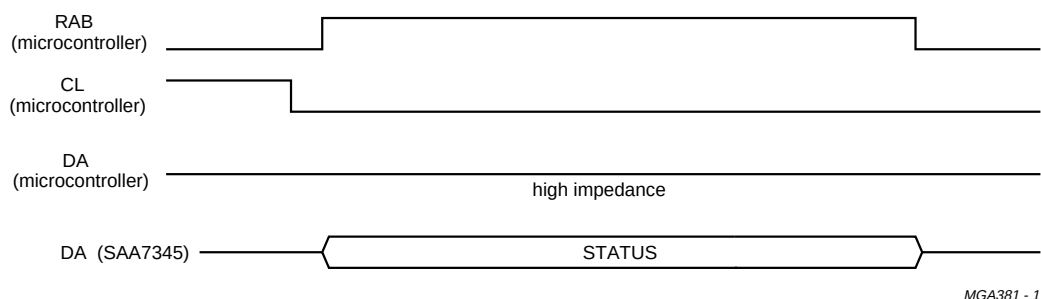
Fig.7 SAA7345 status READ timing.
