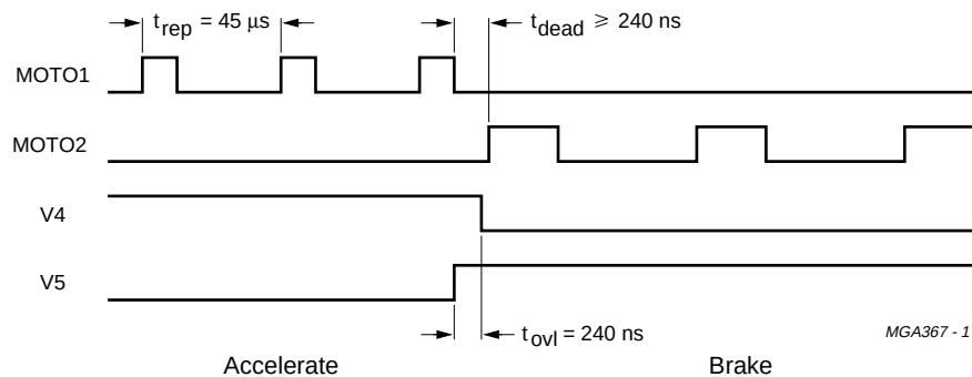
Fig.19 Motor 4-line PWM mode timing.
