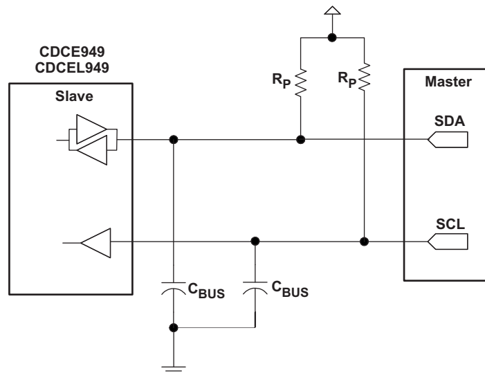
Figure 13. SDA/SCL Hardware Interface
