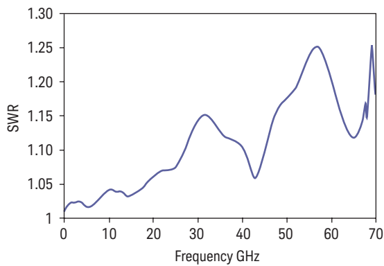
Typical SWR, 10 MHz to 70 GHz (25 ± 10 °C) for N8488A power sensor
