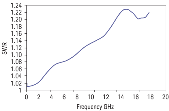
Typical SWR, 10 MHz to 18 GHz (25 ± 10 °C) for N8481H power sensor
