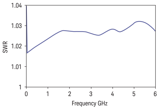
Typical SWR, 100 kHz to 6 GHz (25 ± 10 °C) for N8482A sensor
