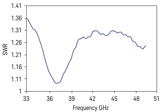
Typical SWR, 33 to 50 GHz (25 ± 10 °C) for N8486AQ power sensor
