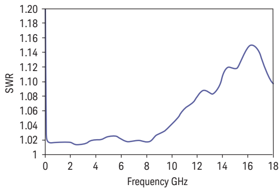
Typical SWR, 10 MHz to 18 GHz (25 ± 10 °C) for N8481A sensor
