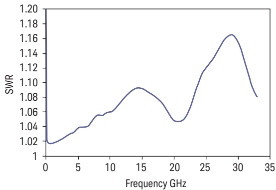
Typical SWR, 10 MHz to 26.5 GHz (25 ± 10 °C) for N8485A sensor
