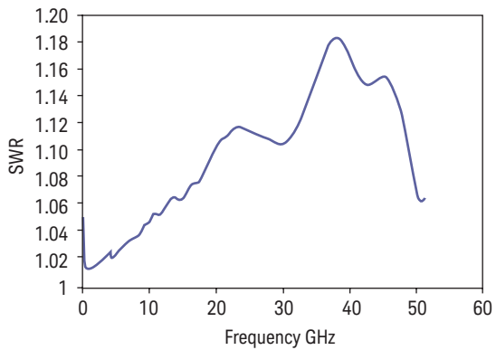
Typical SWR, 50 MHz to 50 GHz (25 ± 10 °C) for N8487A power sensor
