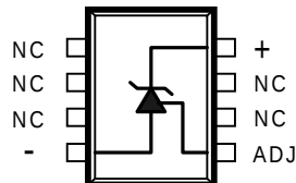
SO-8 Top View
