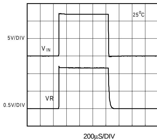
Transient Response
