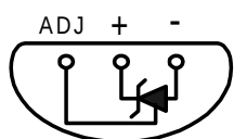
TO-92 Bottom View
