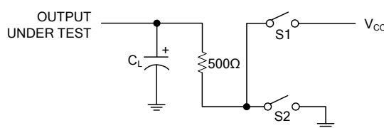
Fig. 4 Driver Enable/Disable Timing Test Load
