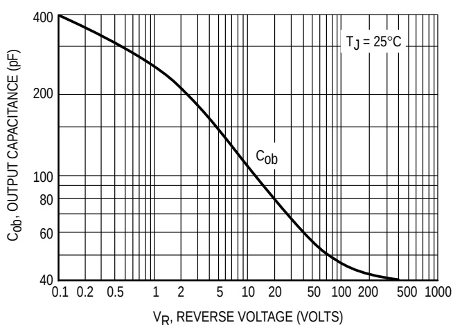
Figure 6. Output Capacitance
