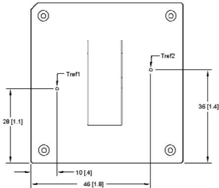
Figure 17. Case ( T_{REF} ) Temperature Measurement Location (top view).
