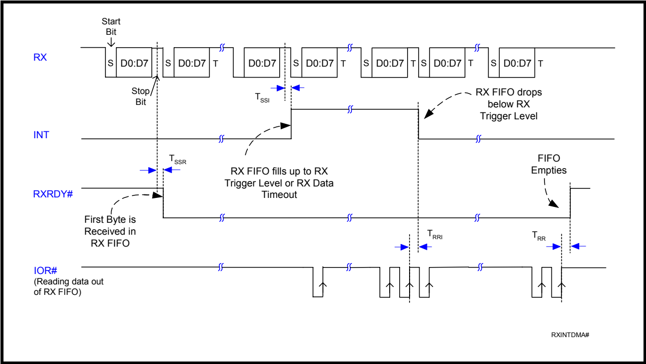
FIGURE 25. RECEIVE READY & INTERRUPT TIMING [FIFO MODE, DMA DISABLED]
