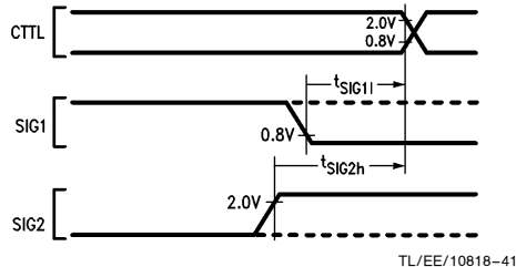
FIGURE 4-3. Input Signals Specification Standard
