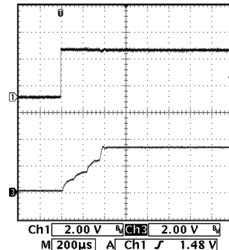
V_{OUT} = 3.3\text{ V} 600-mA Load
