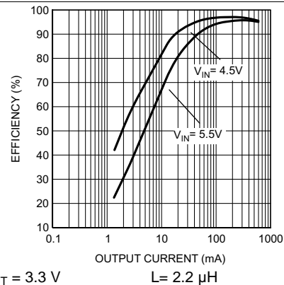
Figure 19. Efficiency vs Output Current (Forced PWM Mode)
