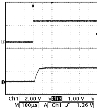
V_{OUT} = 1.2\text{ V} 30-mA Load
