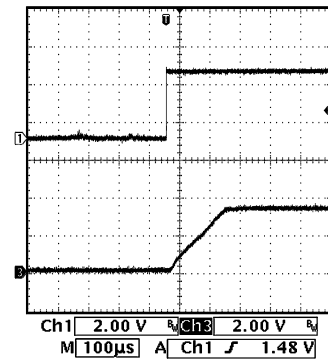
V_{OUT} = 3.3\text{ V} 30-mA load
