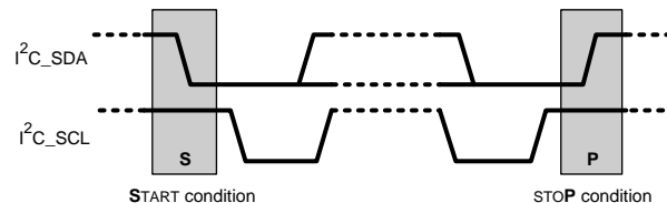
Figure 40. Start and Stop Conditions
