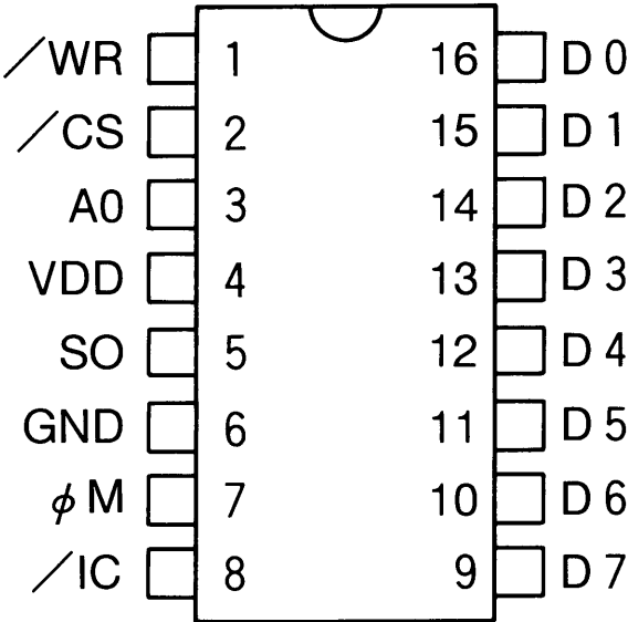
Top View (16pin DIP, 16pin SOP)
