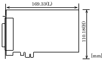
The standard outside dimension (L) is the distance from the end of the board to the outer surface of the slot cover.
