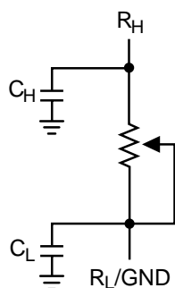
Variable Resistor Equivalent Circuit
