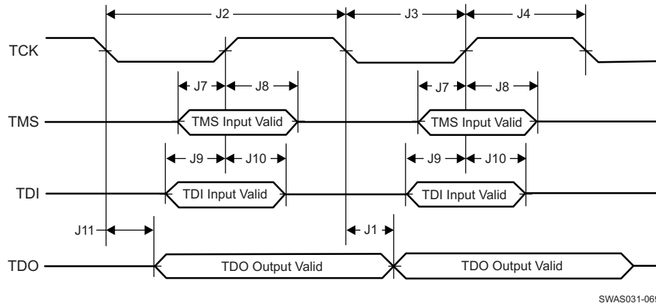
Figure 4-19. JTAG Timing Diagram
