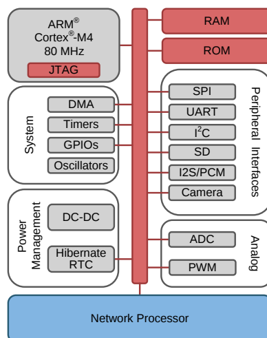
Figure 1-1. CC3220x Hardware Overview
