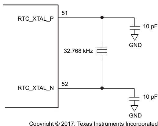
Figure 4-9. RTC Crystal Connections
