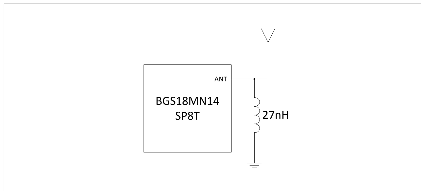
Figure 8: Application circuit
