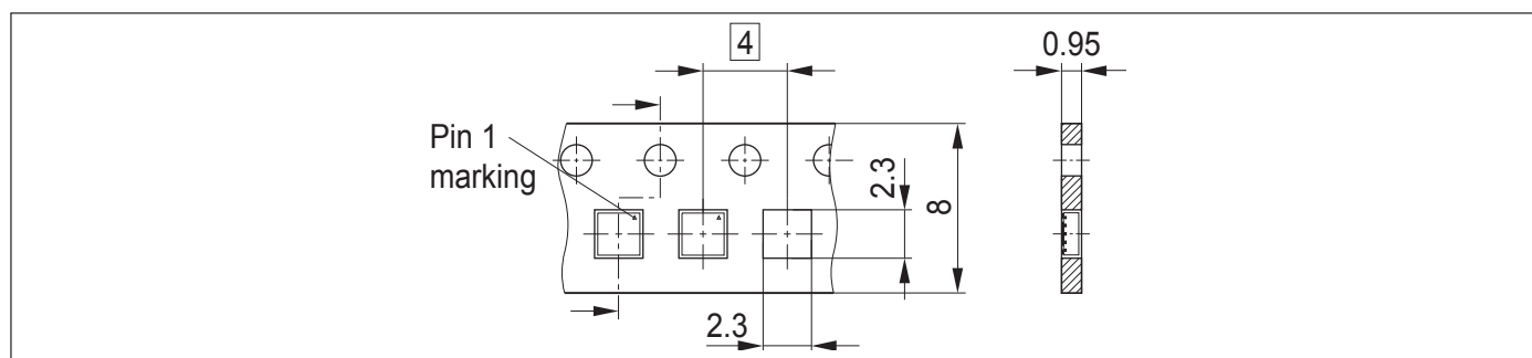
Figure 13: Tape dimensions
