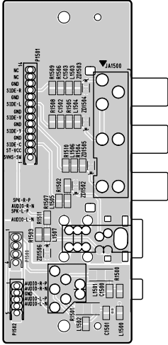
SIDE A/V BOARD BOTTOM (FOIL) SIDE
