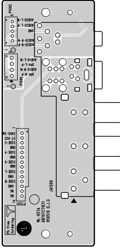
SIDE A/V BOARD TOP (COMPONENT) SIDE
