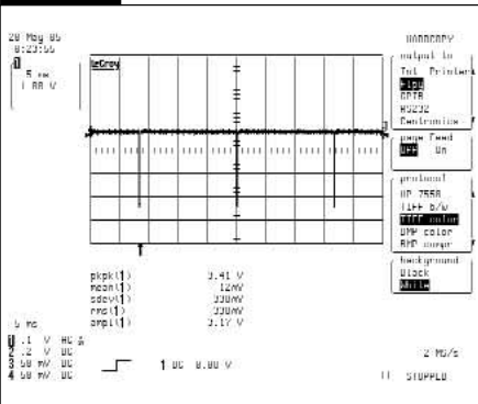
Ref.7-1 PC H Signal Input : IC501, #181
