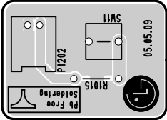
POWER BOARD TOP (COMPONENT) SIDE
