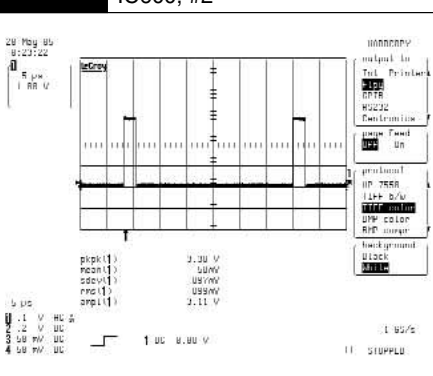
Ref.7 HDMI H Signal output : IC600, #2
