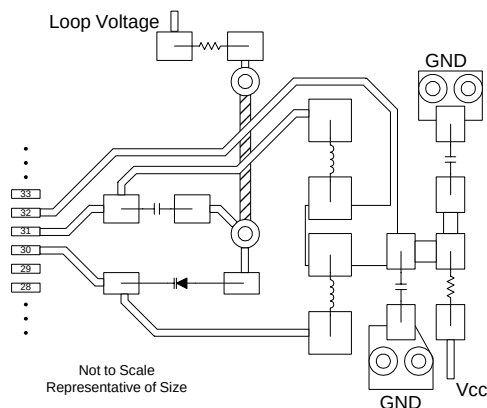
Figure 1. Recommended VCO Layout
