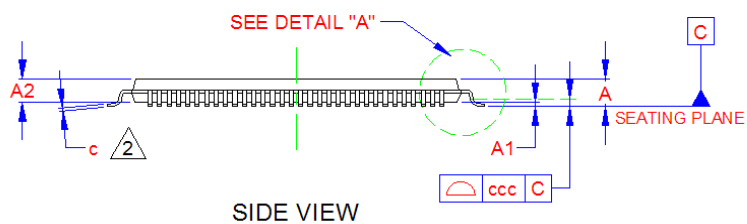
Figure 3 LAN9311 128-VTQFP Package Definition
