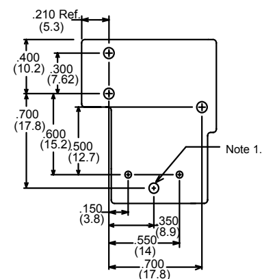
Pin Layout Bottom View
