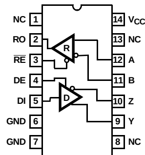
ISL83080E, ISL83083E, ISL83086E (SOIC) TOP VIEW
