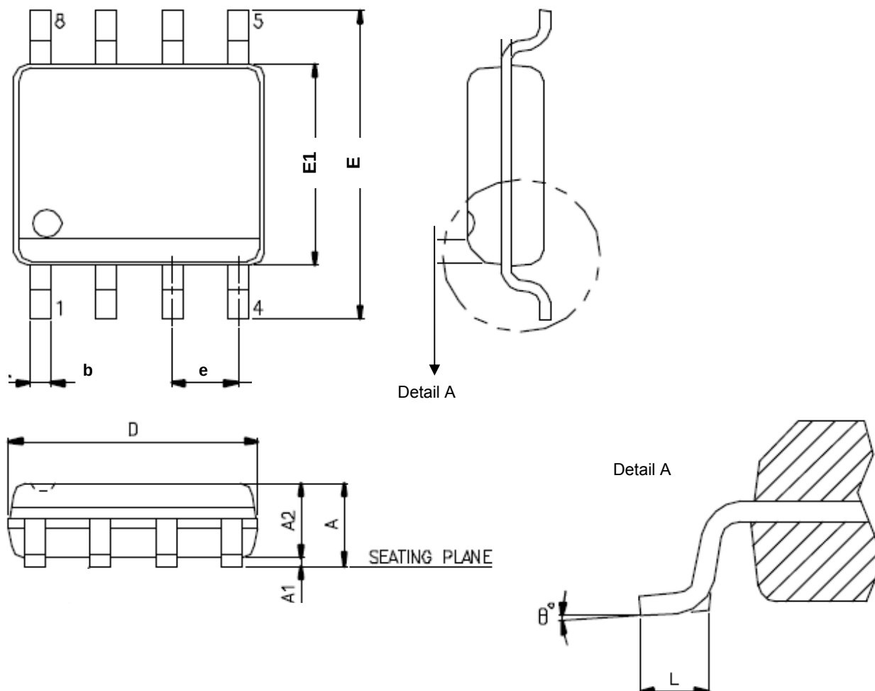
Figure 26. SOP 8 ( 150 mil )
